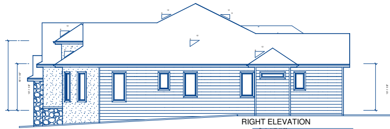
RIGHT ELEVATION Scale 1/4"=1'-0"
