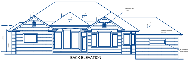
BACK ELEVATION Scale 1/4"=1'-0"
